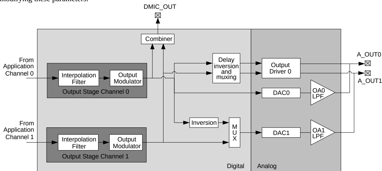
Figure 8. Output Stage
