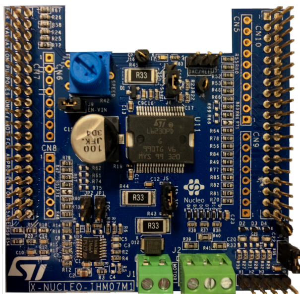
Figure 1. X-NUCLEO-IHM07M1 three-phase brushless DC motor driver expansion board based on L6230 for STM32 Nucleo
