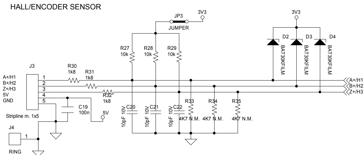
Figure 8. X-NUCLEO-IHM07M1 Hall/Encoder sensor circuit
