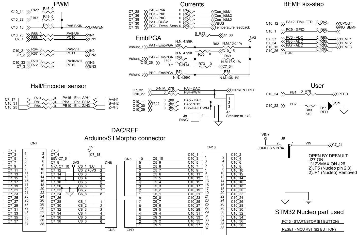
Figure 14. X-NUCLEO-IHM07M1 circuit schematic (4 of 4)
