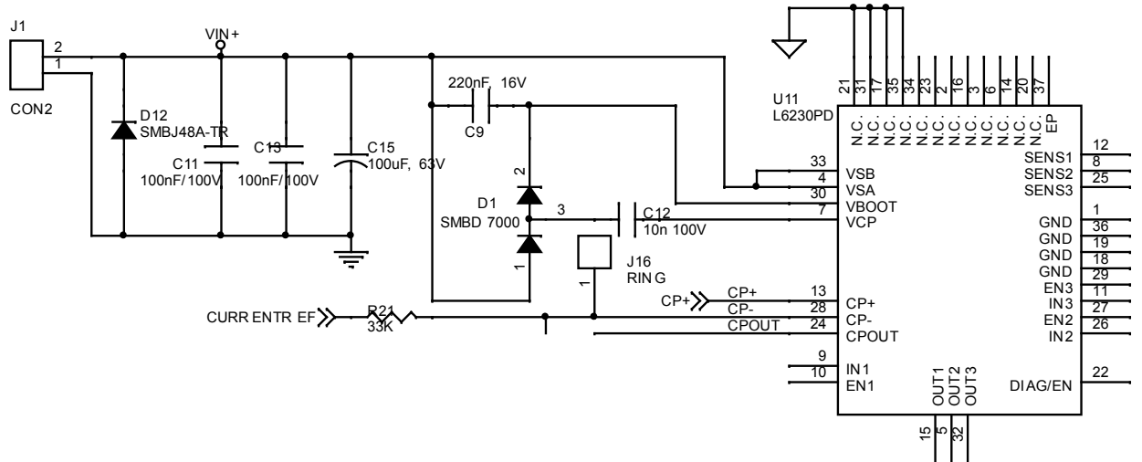
Figure 6. X-NUCLEO-IHM07M1 – charge pump circuit
