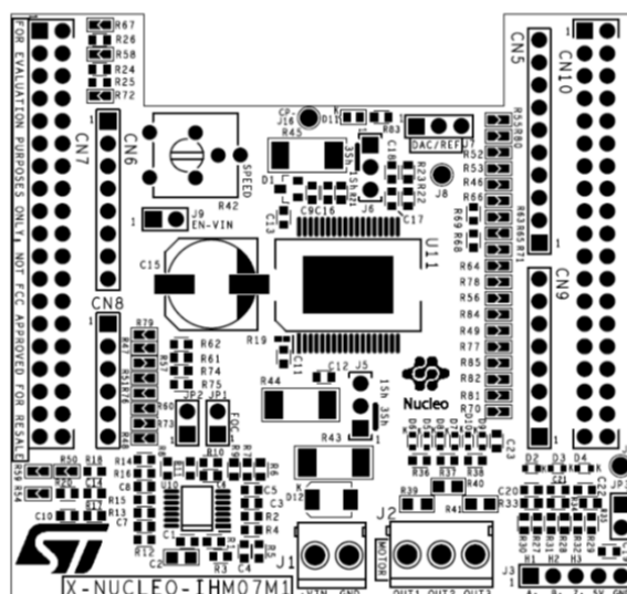
Figure 4. X-NUCLEO-IHM07M1 silk-screen (top layer)
