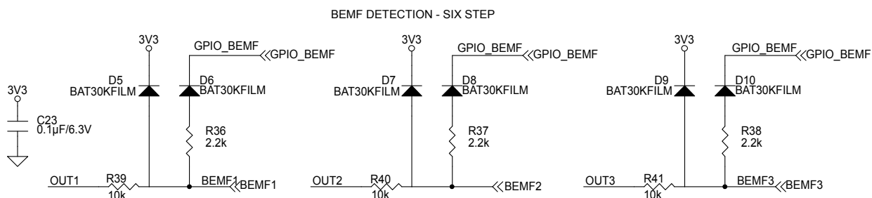
Figure 9. X-NUCLEO-IHM07M1 – BEMF detection circuit
