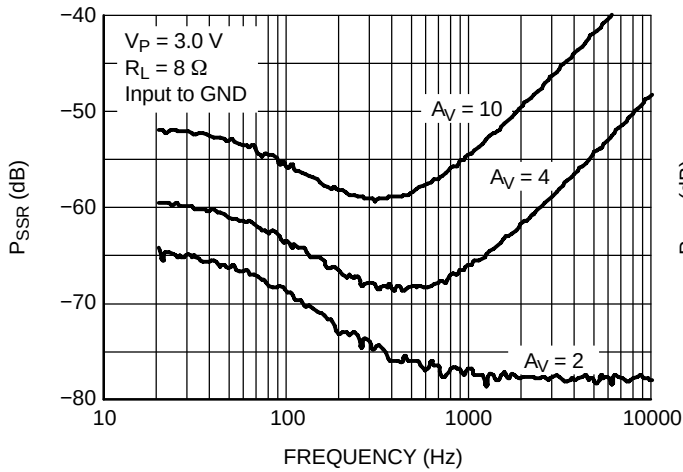
Figure 14. P_{SRR} versus Frequency and Gain @ V_P = 3.0\text{ V}
