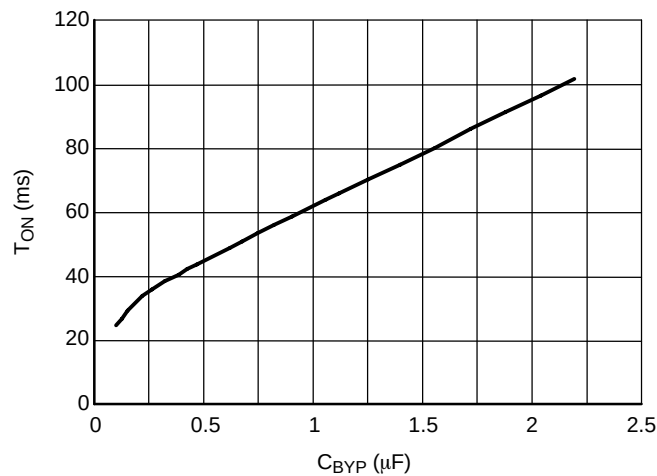
Figure 18. Turn On Time versus C_{BYP} @ V_{BAT} = 3.6\text{ V} , T_A = +25^{\circ}\text{C} , C_{IN} = 100\text{ nF} , R_{IN} = 22\text{ k} , R_F = 110\text{ k}
