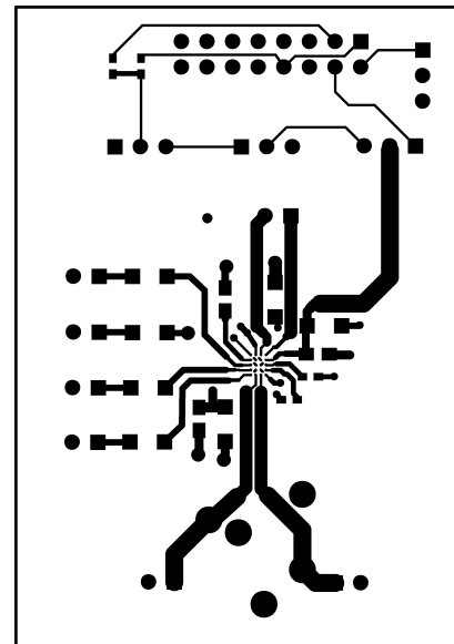
Figure 42. Top Layer
