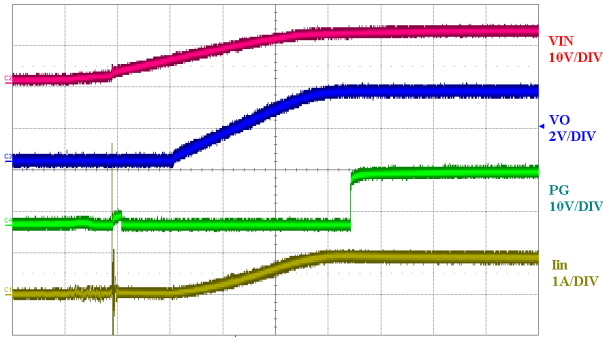
Figure 5. Start-Up into Full Load 1 \text{ms}/\text{DIV}
