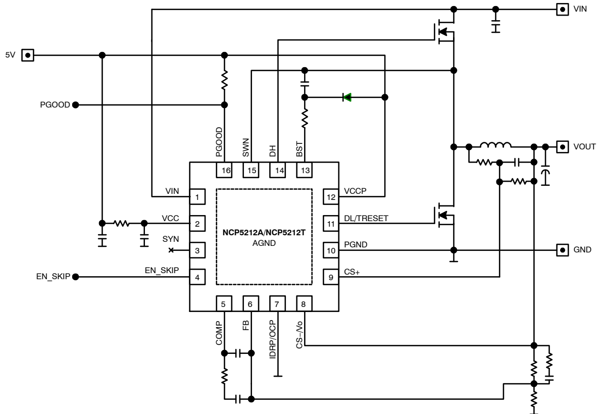
Figure 2. Typical Application Circuit (Single Device Operation)
