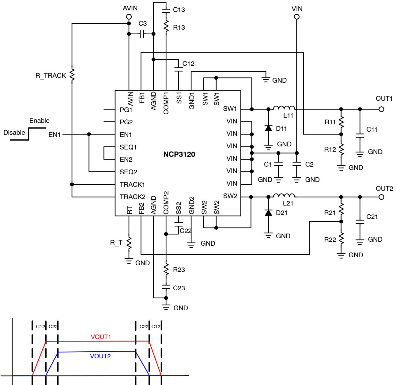
Figure 43. Sequential Configuration
