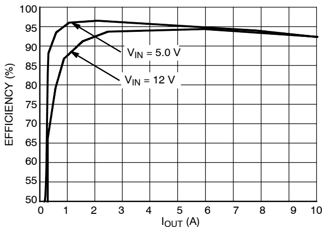
Figure 2. Efficiency
