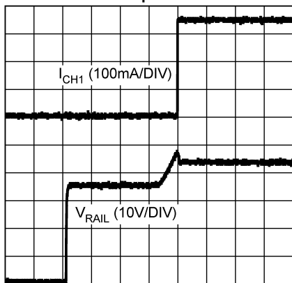
Startup Waveforms
