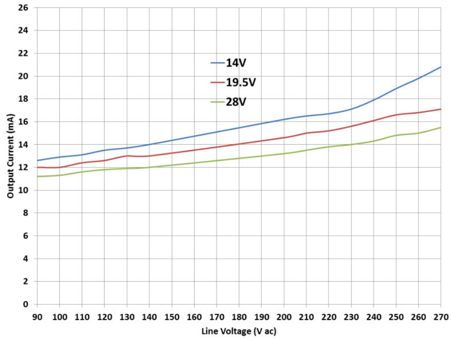
Figure 17. Minimum Load Regulation over Line (NCL30088FLYGEVB only)
