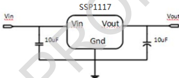
Application circuit of SSP1117 fixed version
