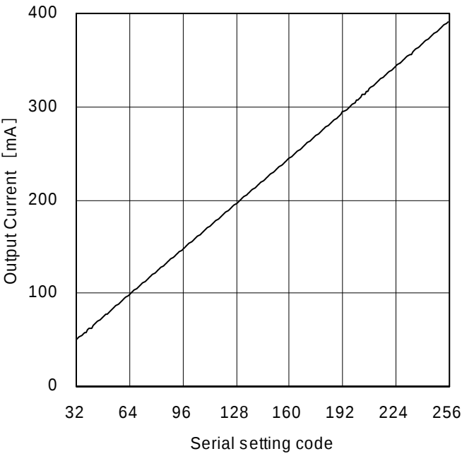
Figure 10. Output Current (Current driver block, RRNF = 1.0\Omega , RL = 5.0\Omega )
