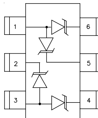
SOT-23 6L (Top View)
