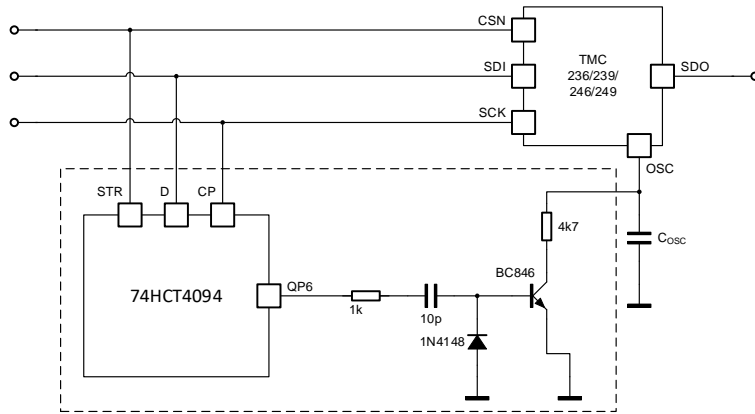
Figure 14.1 Synchronizing the chopper clock
