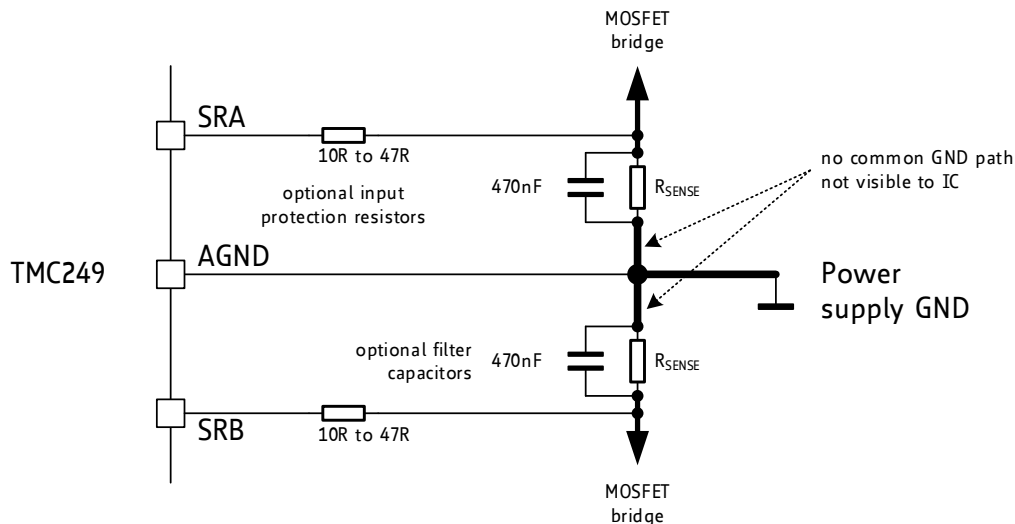
Figure 13.1 Sense resistor grounding and protection components
