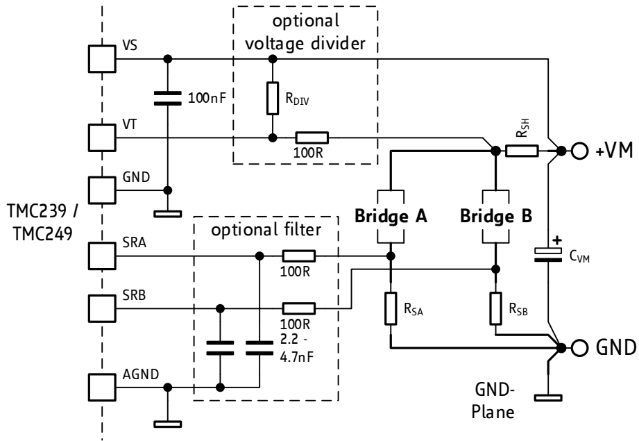
Figure 13.2 Grounding TMC249
