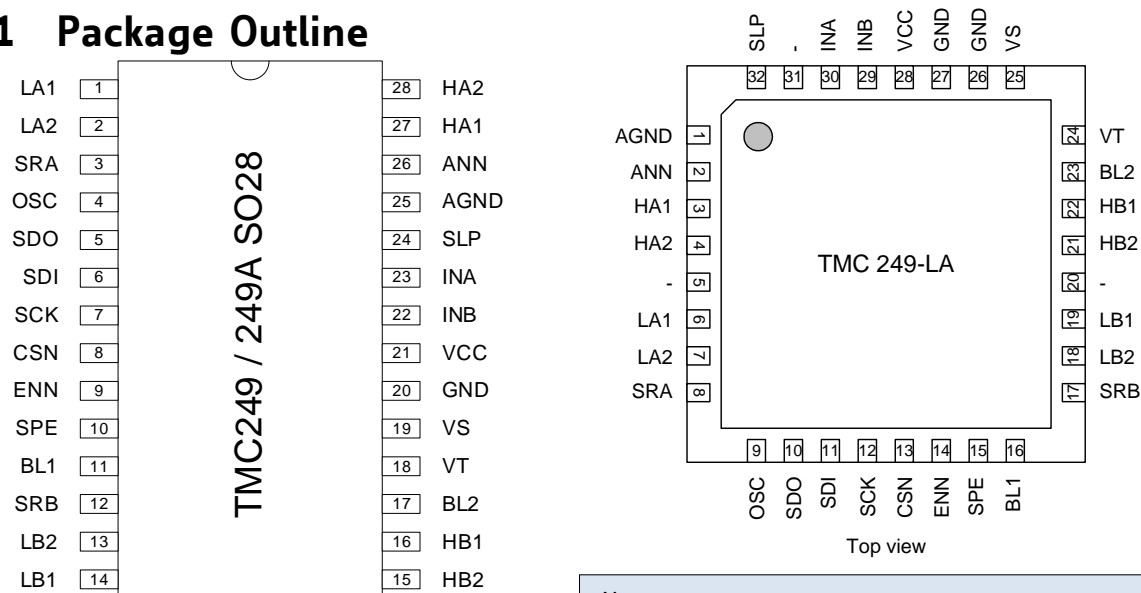
Figure 2.1 TMC249 pin assignments
