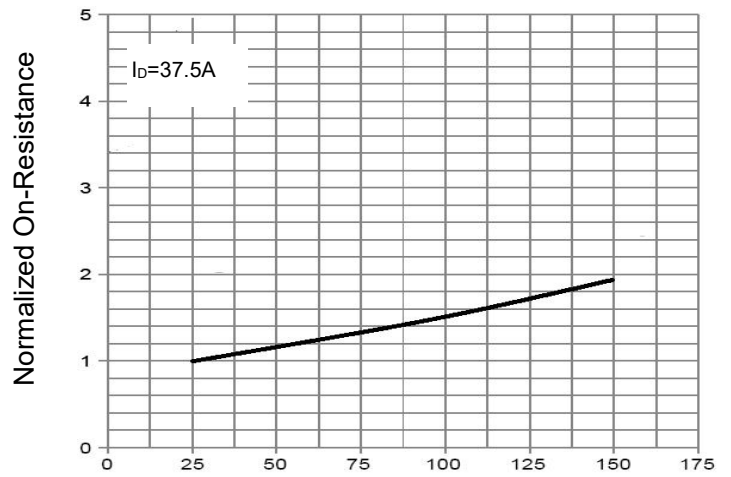
Figure 10 Rdson-Junction Temperature
