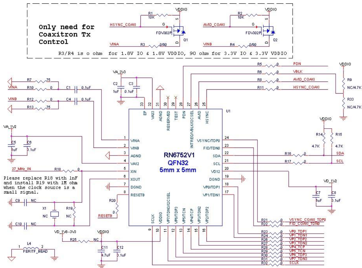
Figure 16: Application schematic
