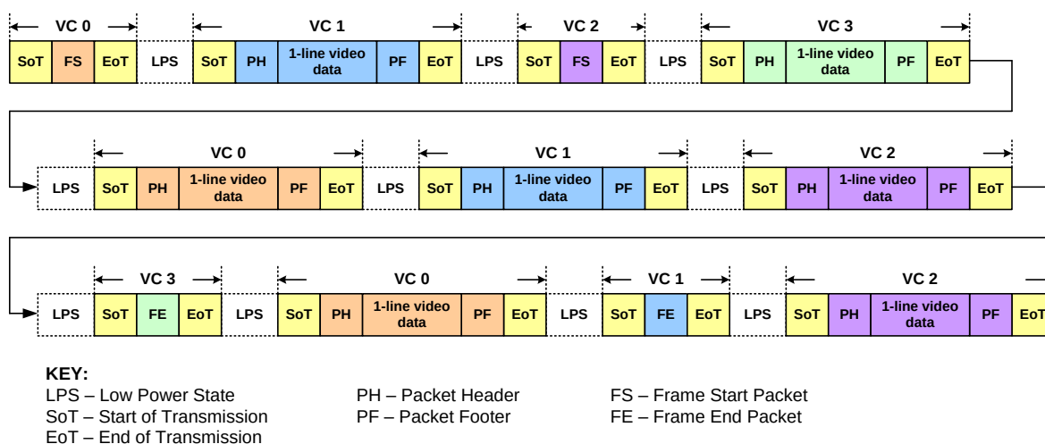
Figure 12: Multi-channel Data Transmission
