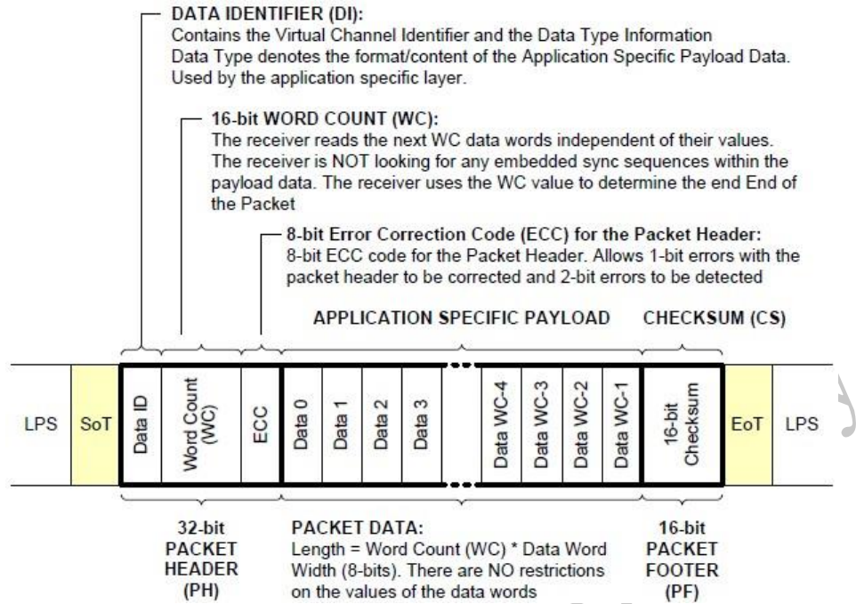
Figure 9: Long Packet Structure
