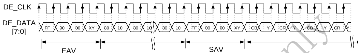
Figure 6: Standard ITU-R BT.656 Format
