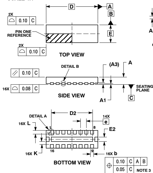
UDFN16 3.5x1.2, 0.4P CASE 517AF ISSUE C
