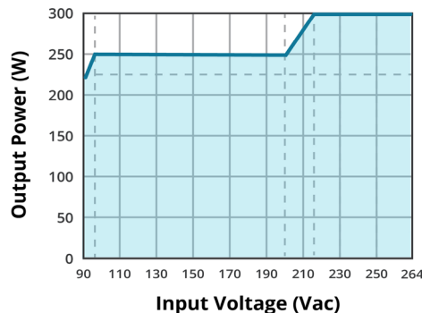
INPUT VOLTAGE DERATING CURVE VOF-300-CNF (natural convection)
