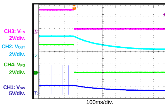
PG Shutdown through EN I_{OUT} = 0A
