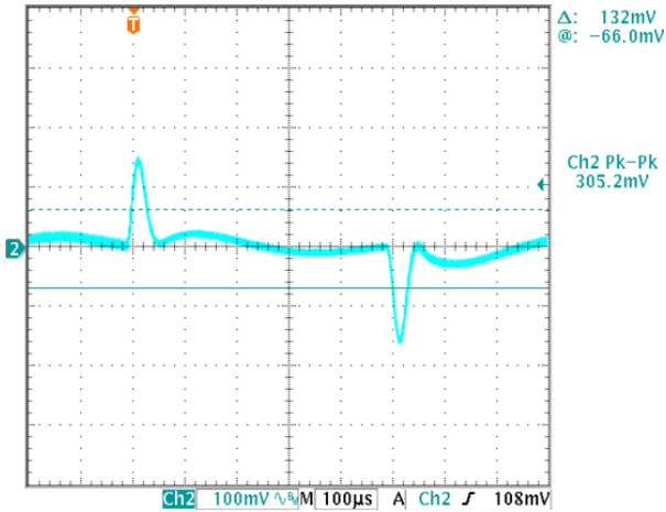
Output Ripple and Noise (Vin=5V, Iout=5A, Vout=3.3V, Cout= 1uF || 10uF, Ta=+25°C)
