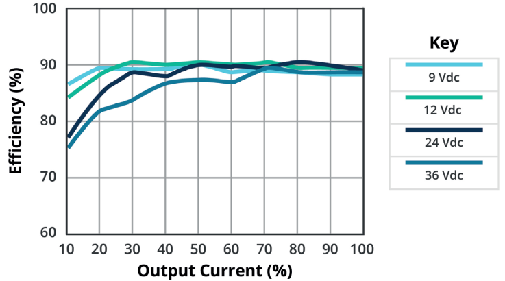
EFFICIENCY VS OUTPUT LOAD PDQ30-Q24-S15-D
