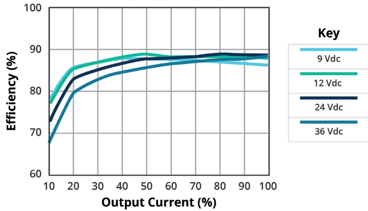
EFFICIENCY VS OUTPUT LOAD PDQ30-Q24-S3-D
