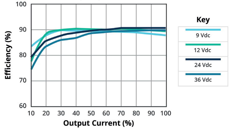
EFFICIENCY VS OUTPUT LOAD PDQ30-Q24-S5-D
