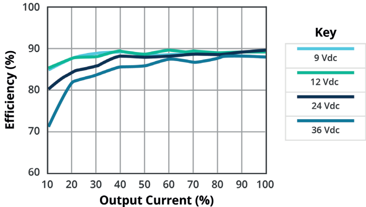
EFFICIENCY VS OUTPUT LOAD PDQ30-Q24-S12-D
