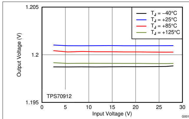
图 6-1. 1.2-V Line Regulation vs V_{IN} and Temperature
