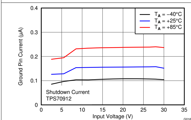
图 6-15. GND Current vs V_{IN} and Temperature
