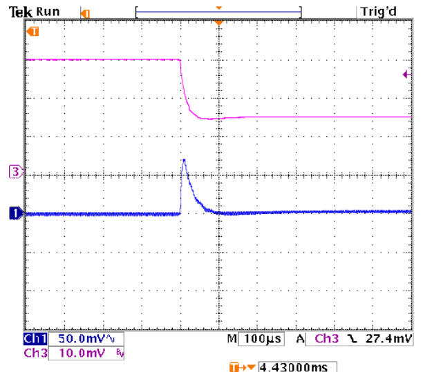
Step Load Transient Response (VIN=12V, Vout=5V, Cload=0, Iout=3A to 1.5A) Trace 1=Vout, 50 mV/div. Trace 3=Iout, 1A/div.
