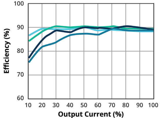
EFFICIENCY VS OUTPUT LOAD PDQ30-Q24-S15-D
