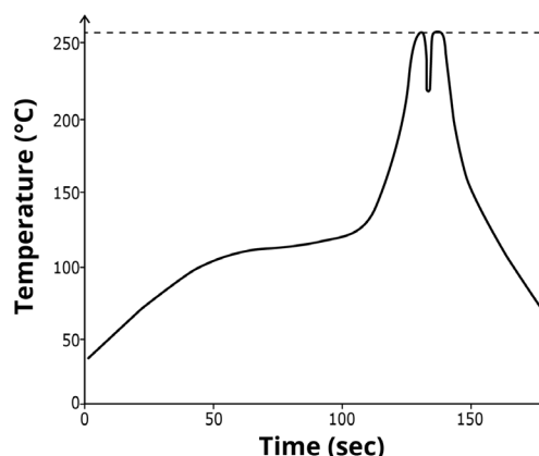
WAVE SOLDERING PROFILE
