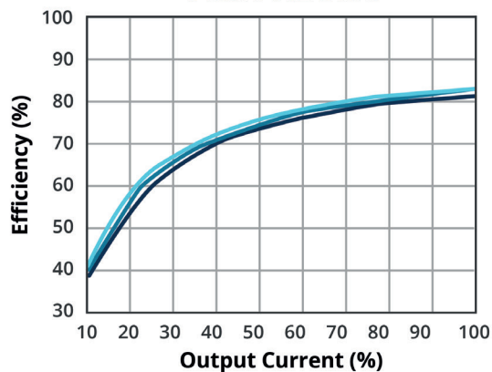
EFFICIENCY VS OUTPUT LOAD PCSA1-S12-S15-S
