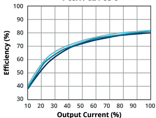
EFFICIENCY VS OUTPUT LOAD PCSA1-S24-S5-S
