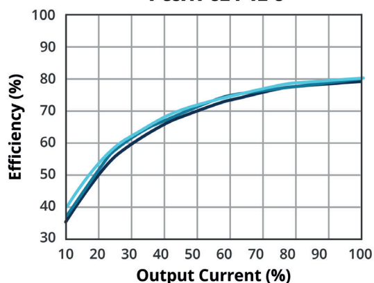
EFFICIENCY VS OUTPUT LOAD PCSA1-S24-S12-S
