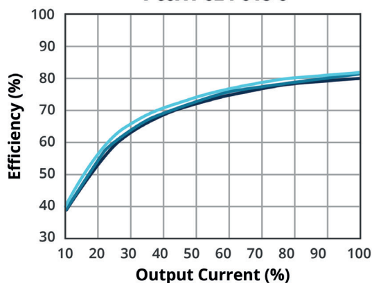
EFFICIENCY VS OUTPUT LOAD PCSA1-S24-S15-S
