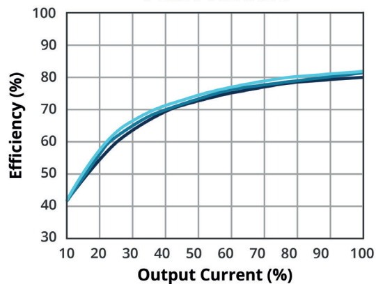
EFFICIENCY VS OUTPUT LOAD PCSA1-S12-S12-S
