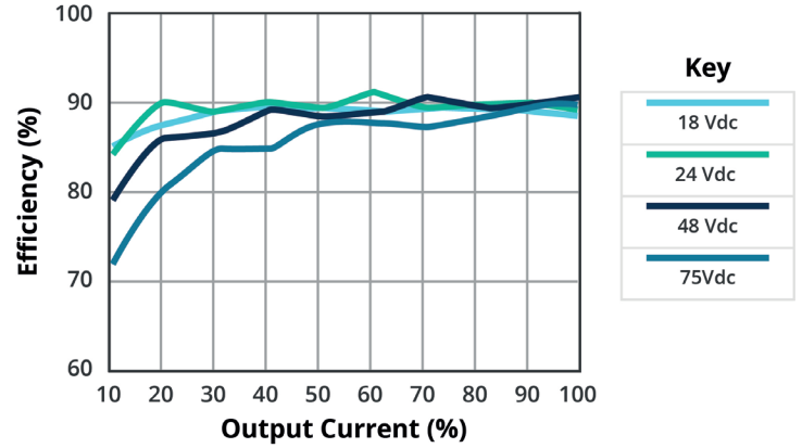
EFFICIENCY VS OUTPUT LOAD PDQ30-Q48-S15-D
