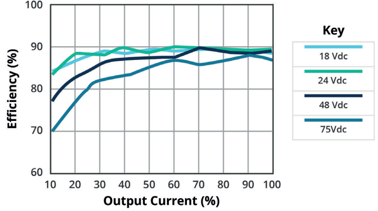
EFFICIENCY VS OUTPUT LOAD PDQ30-Q48-D15-D
