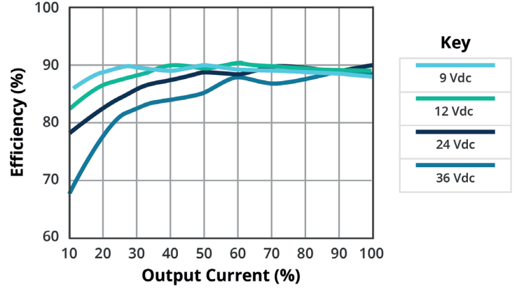
EFFICIENCY VS OUTPUT LOAD PDQ30-Q24-D15-D
