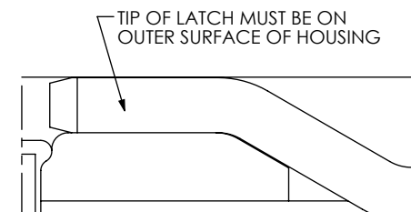
DETAIL 'A' SCALE 16:1
