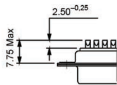
Solder Buckets
