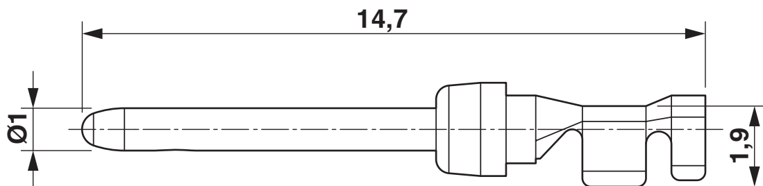
Dimensional drawing
