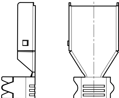
REAR SHELL
