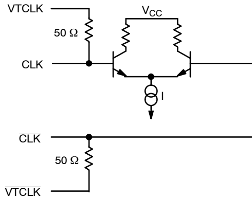
Figure 4. Input Structure
