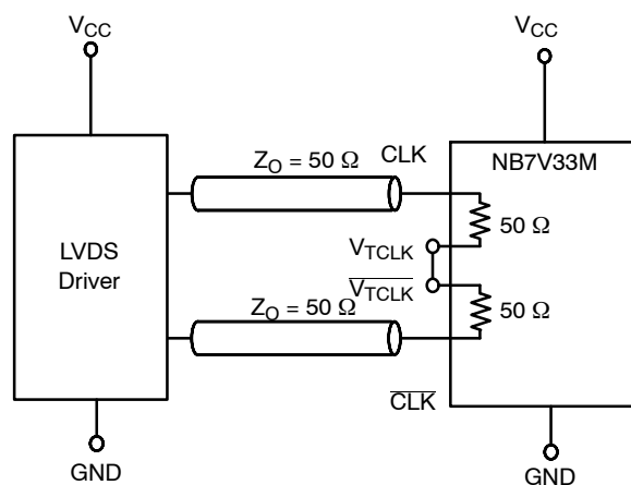
Figure 12. LVDS Interface
