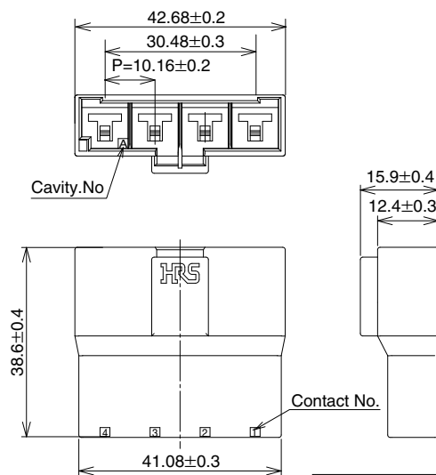
Inline plug with 4 pos.
