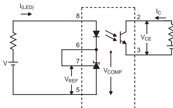
Figure 7. CTR, V_{CE(sat)} Test Circuit
