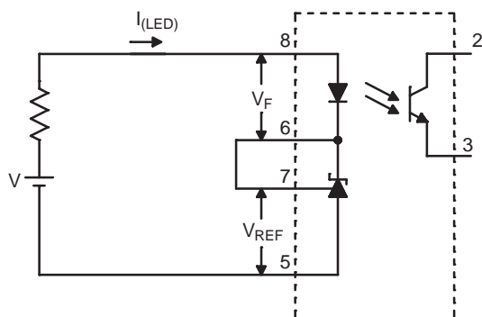
Figure 2. V_{REF} , V_F , I_{LED} (min.) Test Circuit
