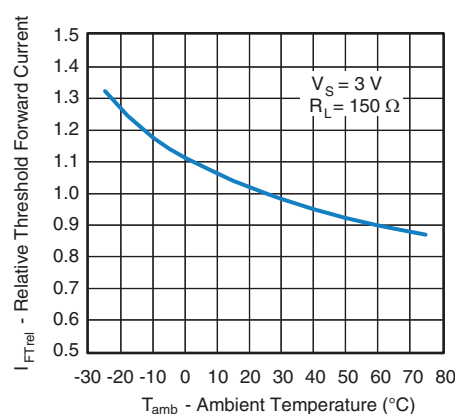
Fig. 7 - Relative Threshold Forward Current vs. Ambient Temperature
