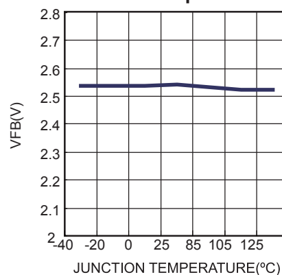
Feedback Voltage vs. Junction Temperature
