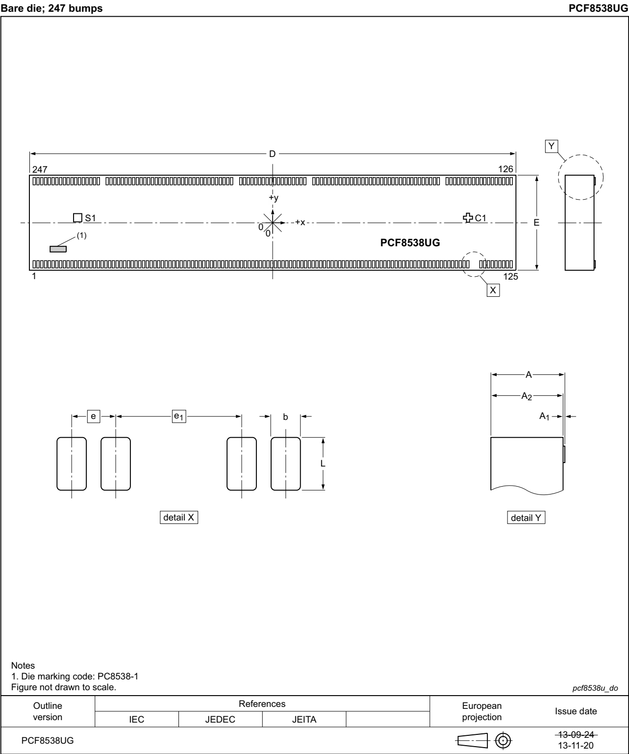
Fig 64. Bare die outline of PCF8538UG
