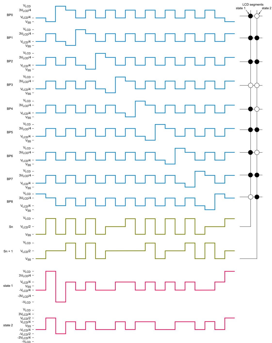
Fig 32. Waveforms for 1:9 multiplex drive mode with 1/4 bias and line inversion mode (n = 1)
