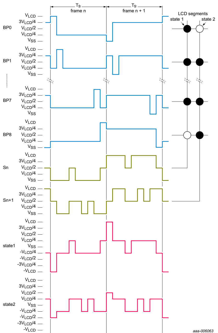
Fig 33. Waveforms for 1:9 multiplex drive mode with 1/4 bias and frame inversion mode
