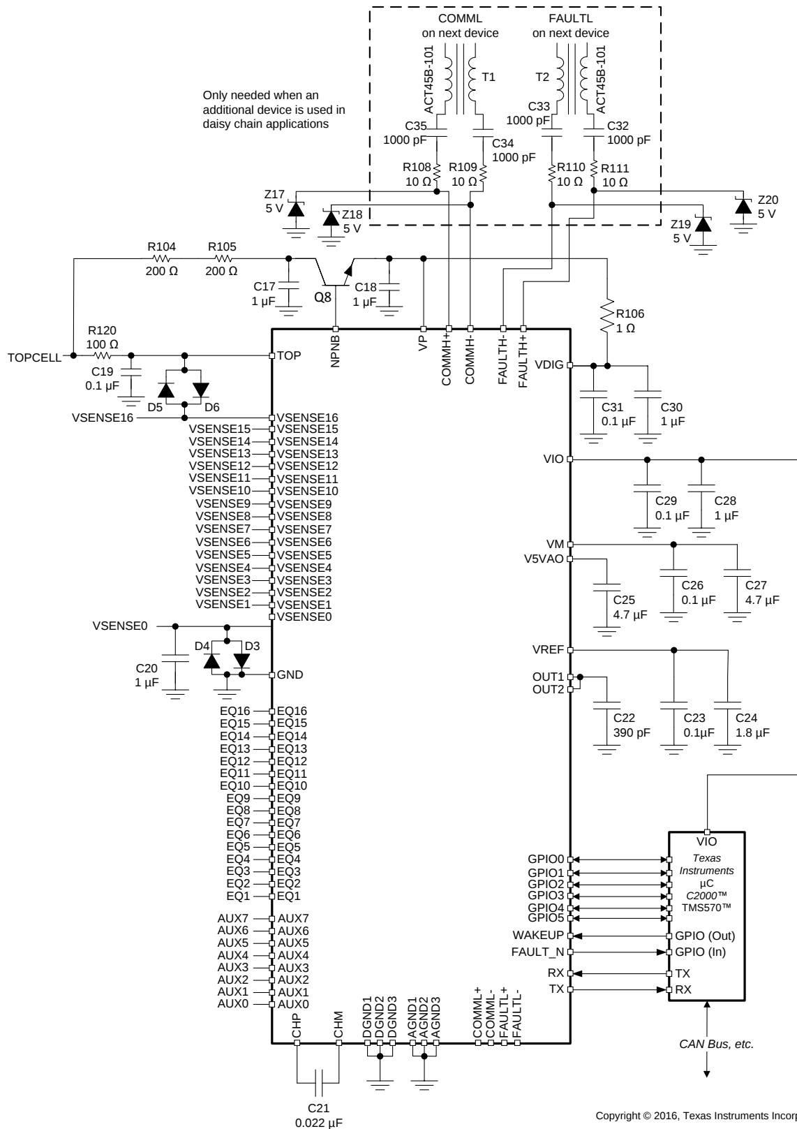
Figure 36. Main Device
