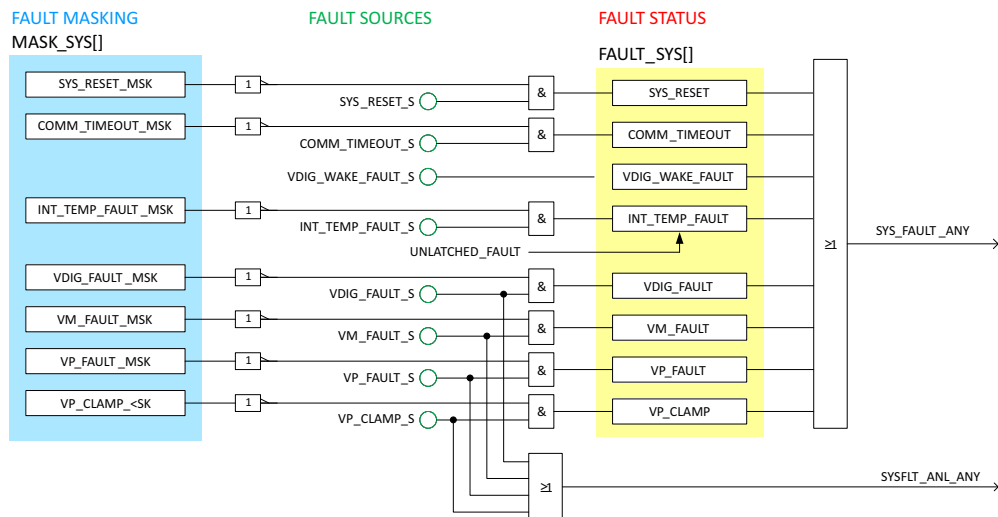
Figure 22. System Faults
