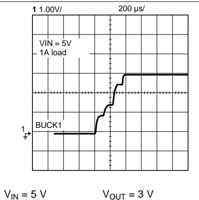
Figure 5. Start-Up of Buck 1
