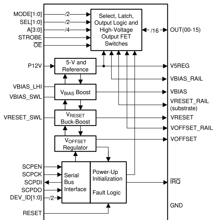
Block Diagram
