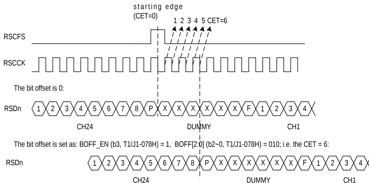
Figure 35. Receive Bit Offset in T1/J1 Mode
