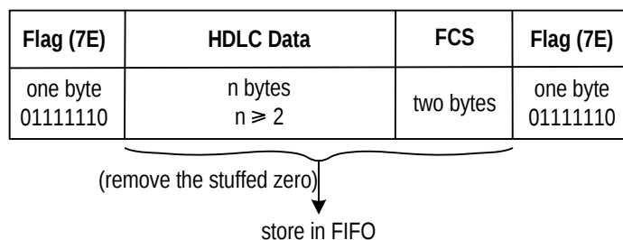
Figure 5. HDLC Packet
