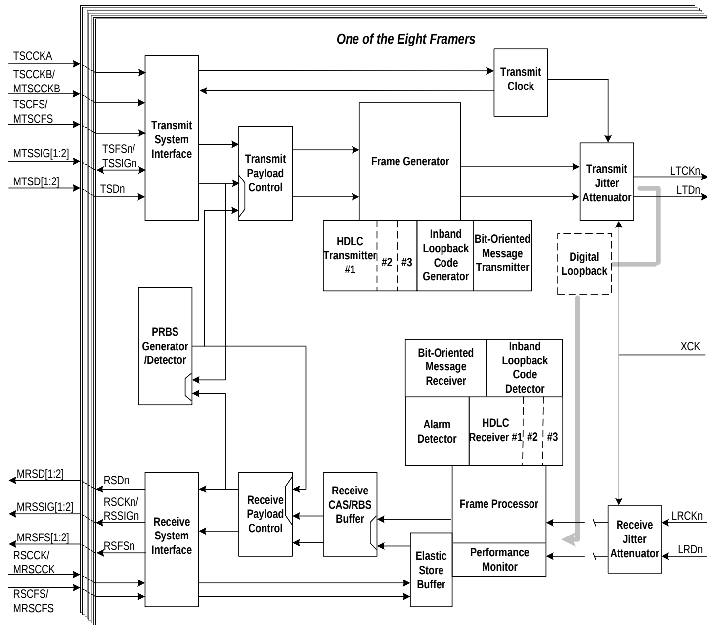
Figure 71. Digital Loopback
