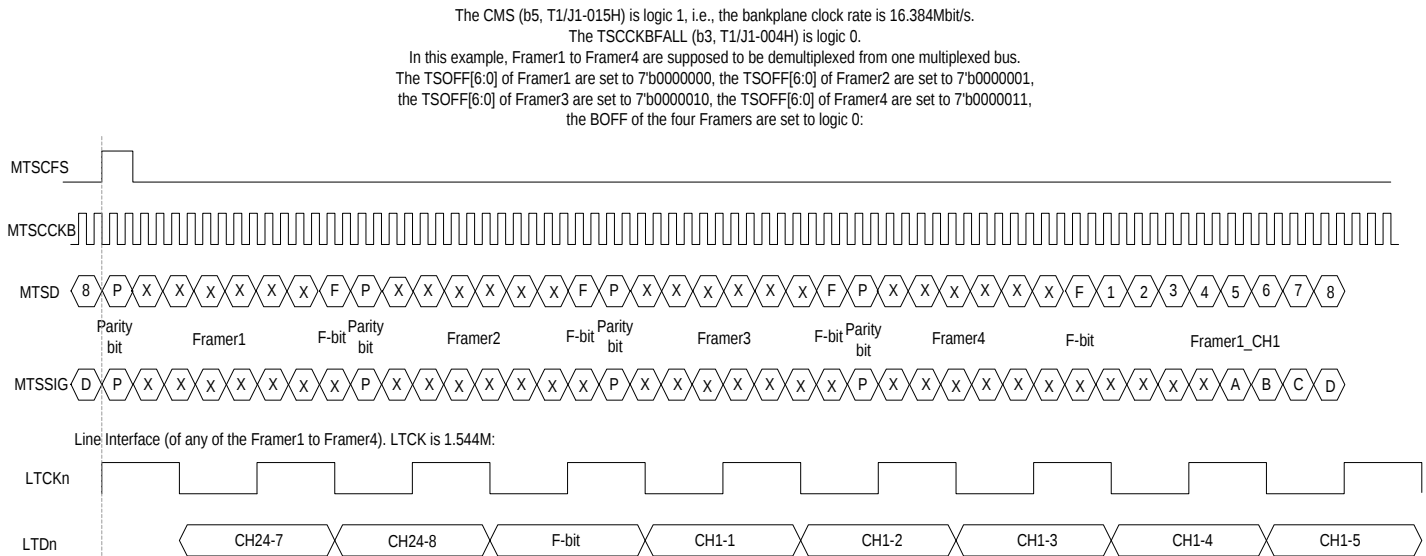
Figure 62. T1/J1 Transmit Multiplexed Mode - Functional Timing Example 2
