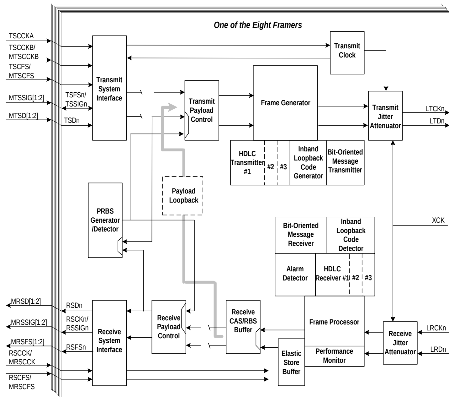
Figure 72. Payload Loopback
