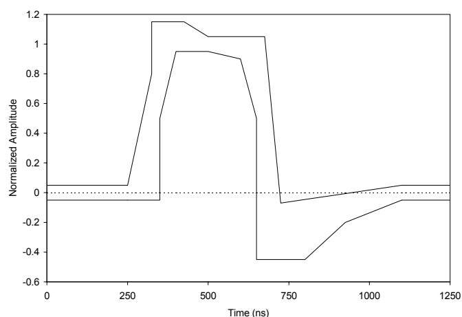
Figure-15 DSX-1 Waveform Template
