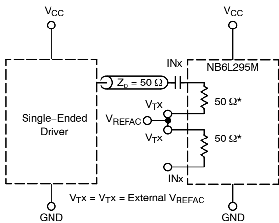
Figure 21. Capacitor-Coupled Single-Ended Interface ( V_{TX}/\sqrt{V_{TX}} Connected to External V_{REFAC} ; V_{REFAC} Bypassed to Ground with 0.1 \mu F Capacitor)
