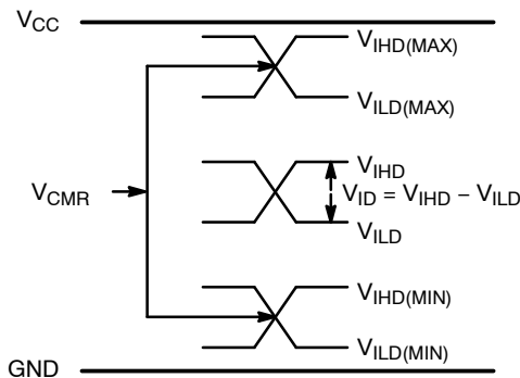
Figure 15. V_{CM} Diagram
