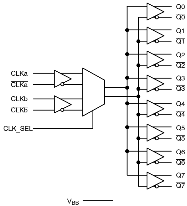
Figure 2. Logic Symbol
