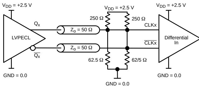
Figure 31. CLK / \overline{\text{CLK}} Input Driven by 2.5 V LVPECL Driver (Thevenin Parallel Termination)
