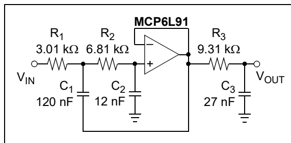
FIGURE 4-5: Chebyshev Filter.
