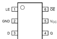
Figure 1. SC88 (Top View)
