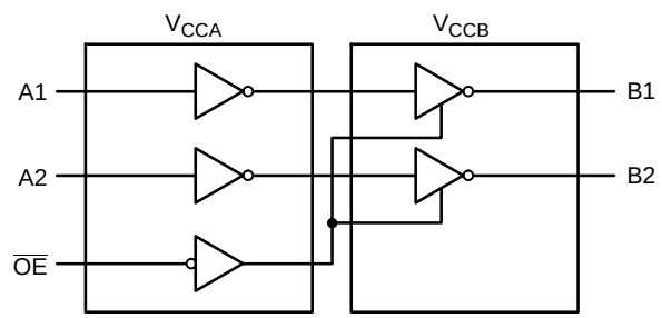
Figure 1. Logic Diagram
