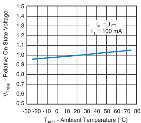
Fig. 4 - Relative On-State vs. Ambient Temperature
