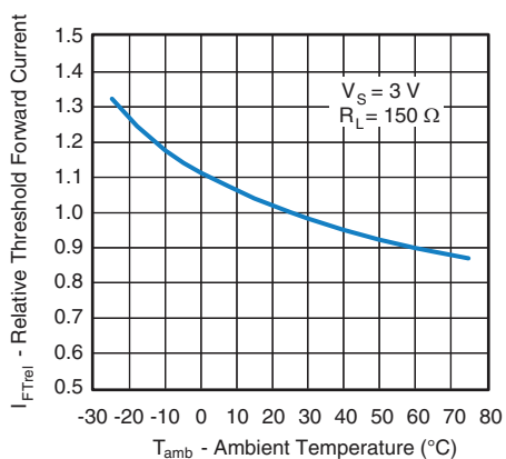
Fig. 3 - Relative Threshold Forward Current vs. Ambient Temperature
