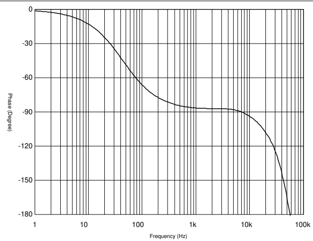
Figure 10-3. Converter Open Loop Bode Plot - Phase
