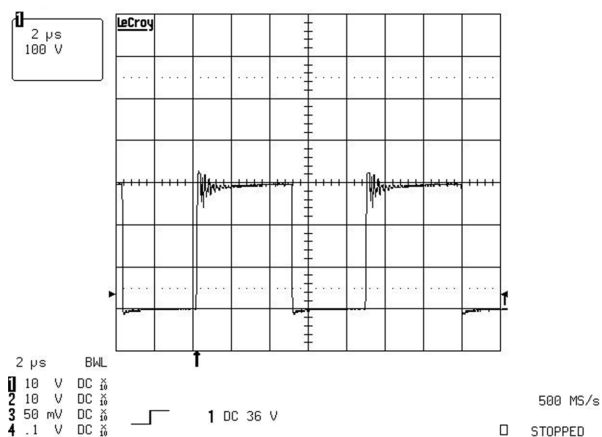
Figure 10-7. Primary Side MOSFET Drain to Source Voltage at 120-V AC Input (100 V/div)
