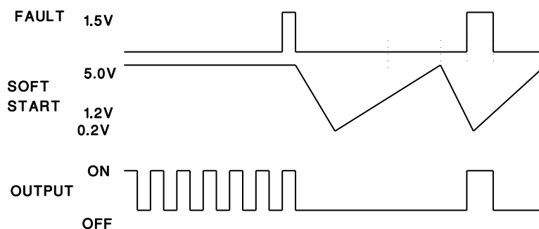
Figure 9-19. IC Behavior at Repetitive Fault
