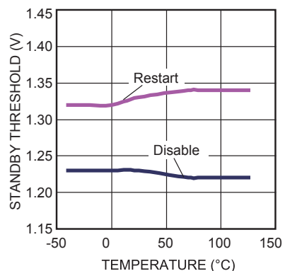
Standby Threshold vs. T_J
