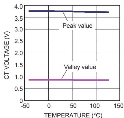
Oscillator Ramp vs. T_J
